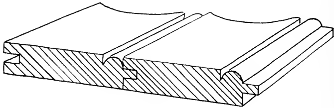
BEADED JOINT
